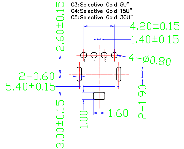
RECOMMENDED PCB LAYOUT GENERAL TOLERANCES: \pm 0.05
